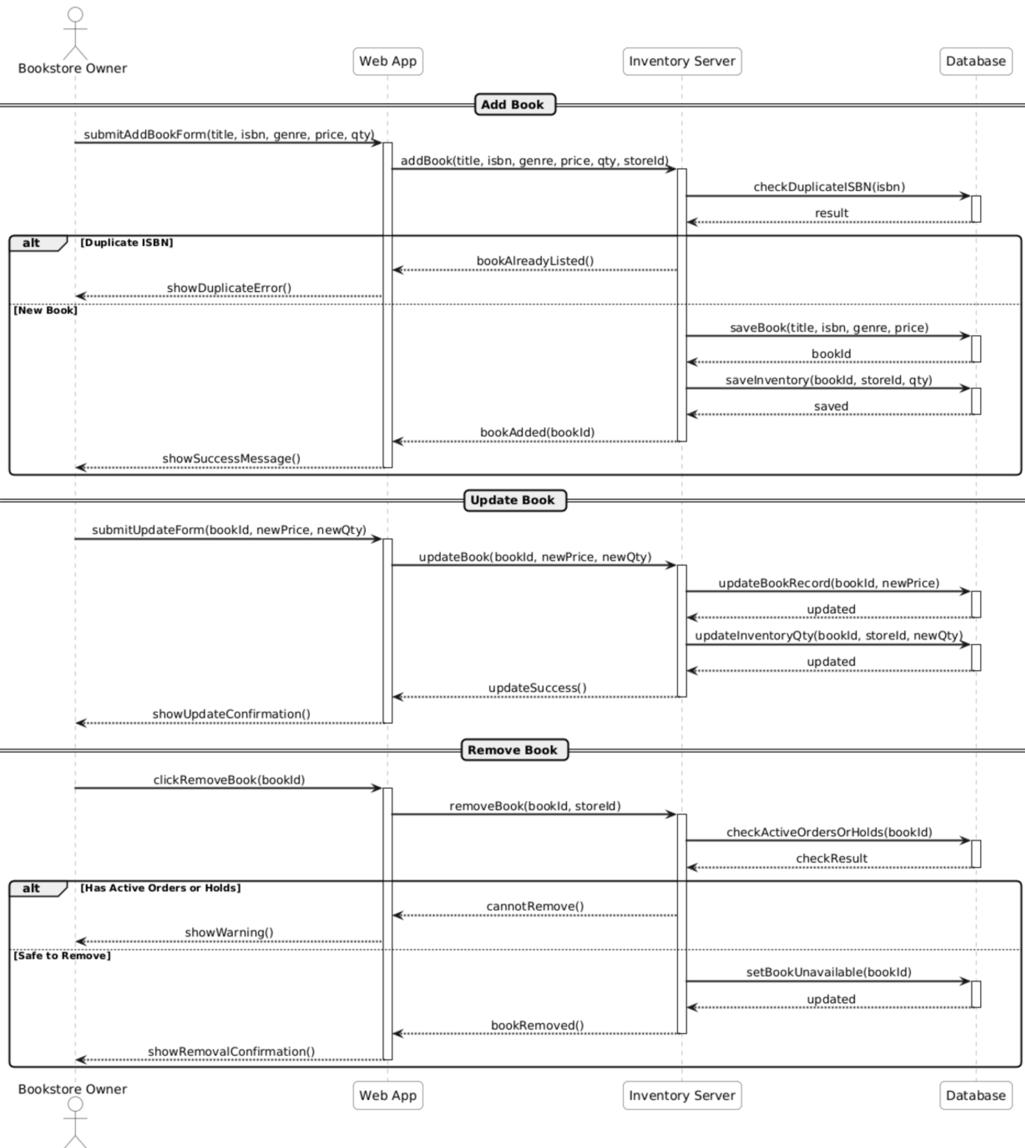
Sequence Diagram 04: Manage Inventory
