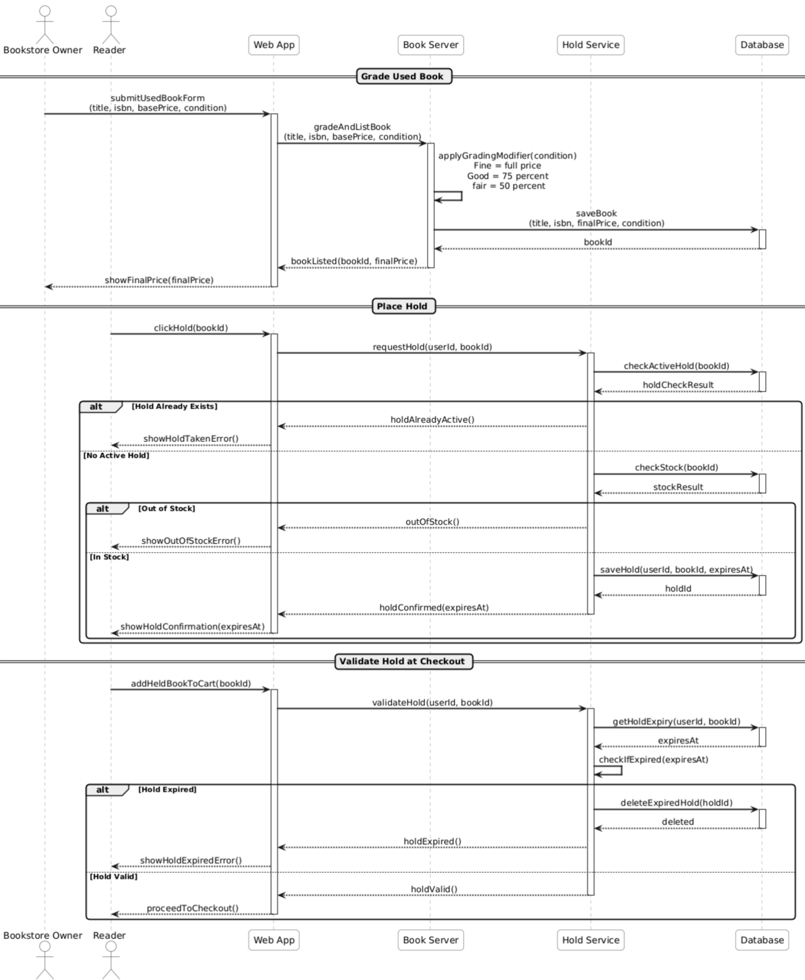
Sequence Diagram 05: Grade Used Book and Place Hold on Shelf
