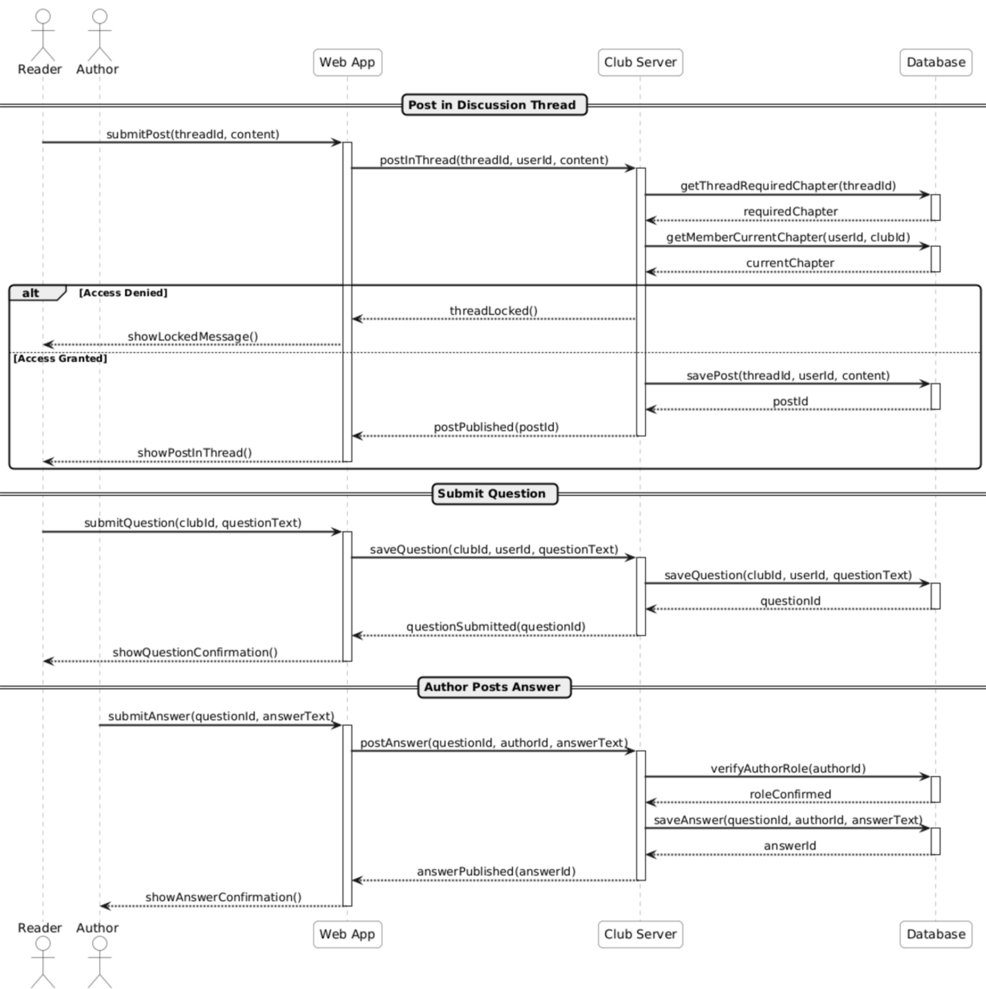
Sequence Diagram 10: Author Q&A and Discussion Threads
