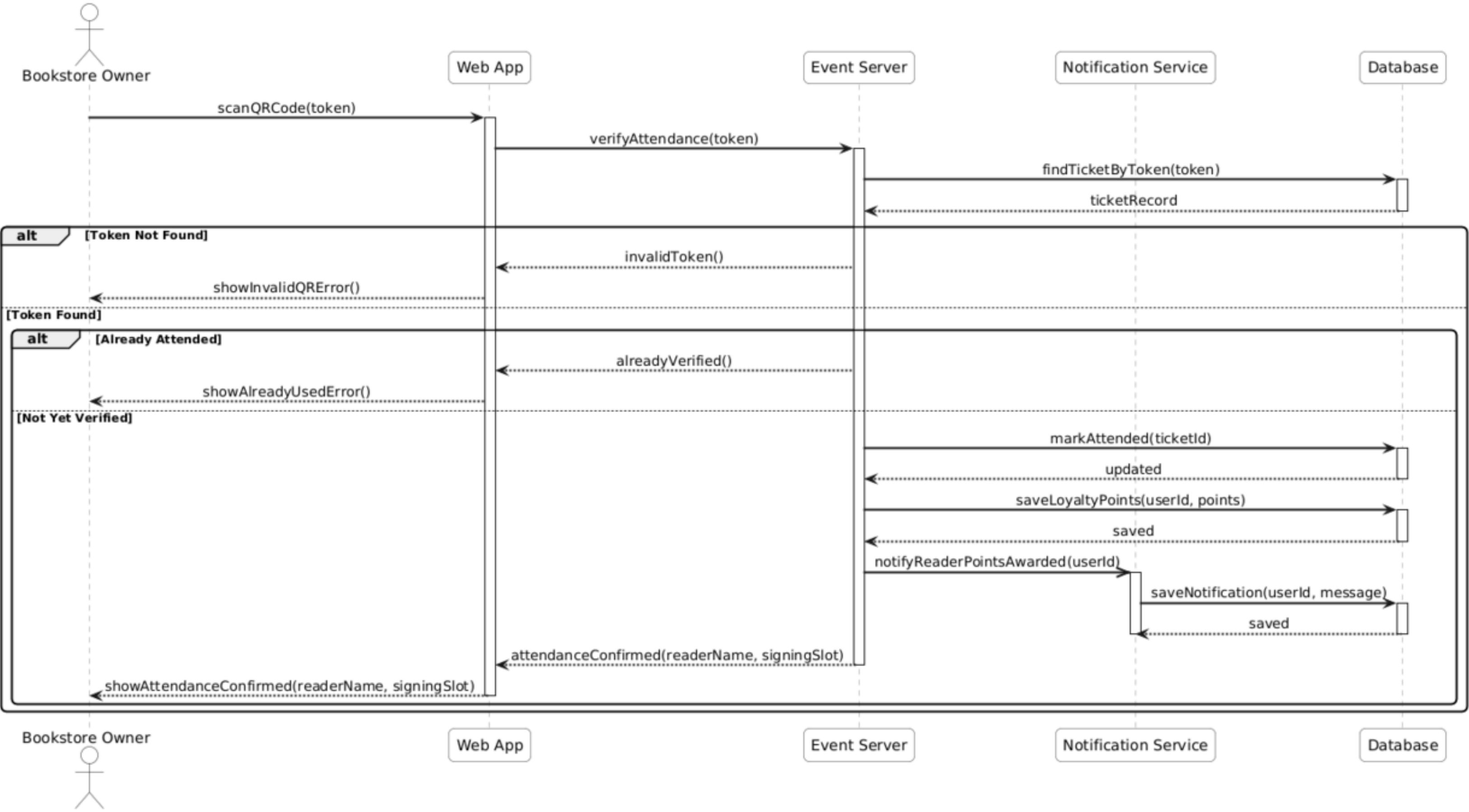
Sequence Diagram 15: Verify Event Attendance
