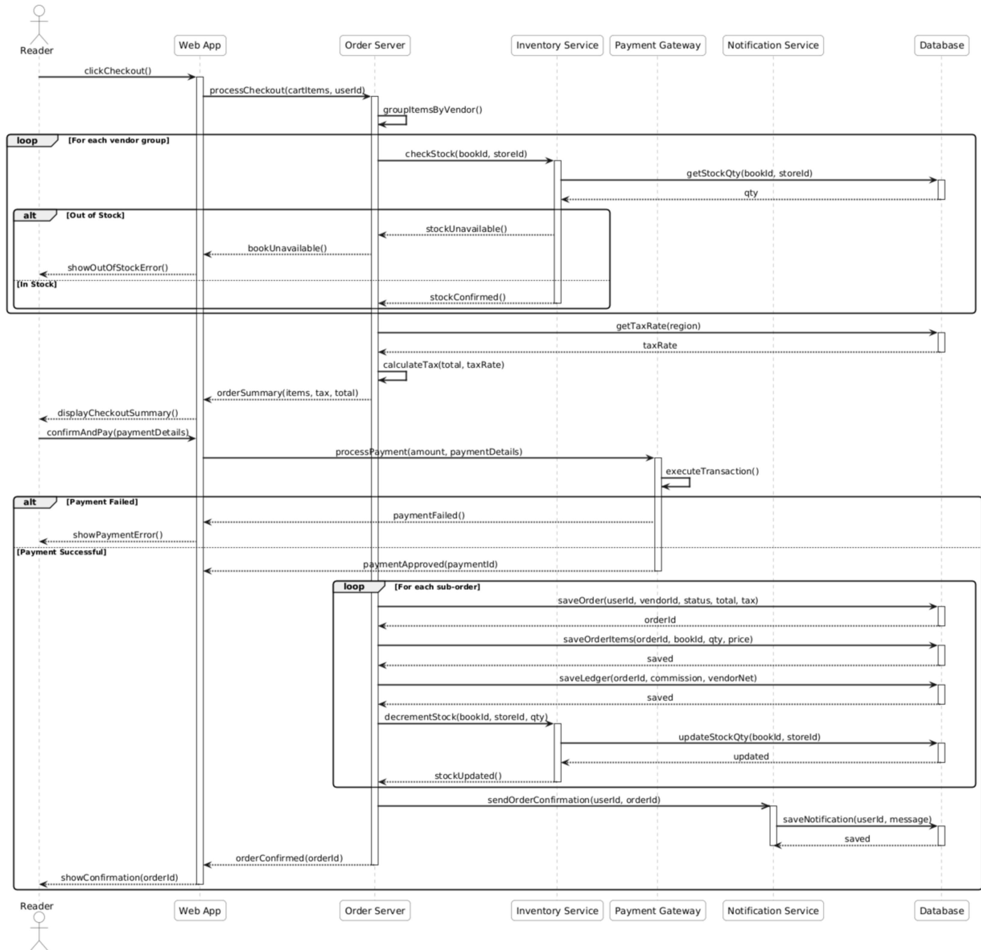
Sequence Diagram 02: Place Order - Click and Collect
