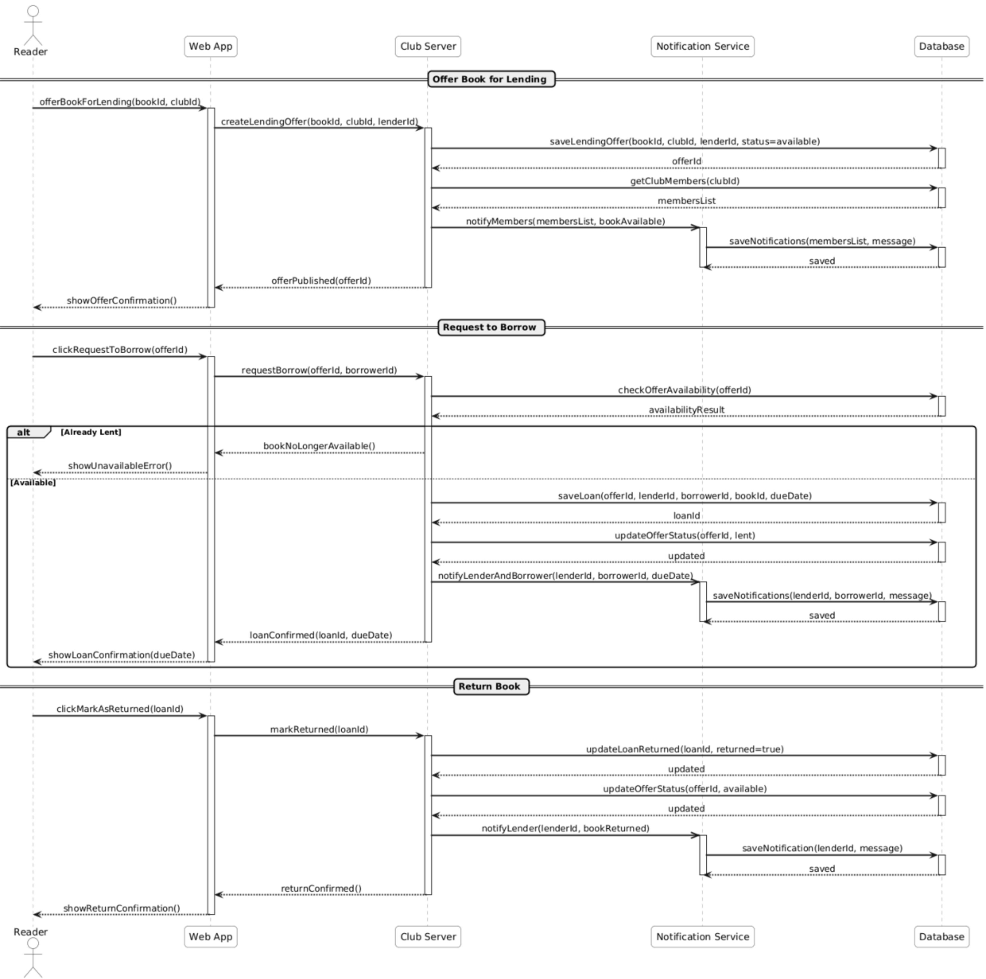
Sequence Diagram 12: Lend and Borrow Physical Book
