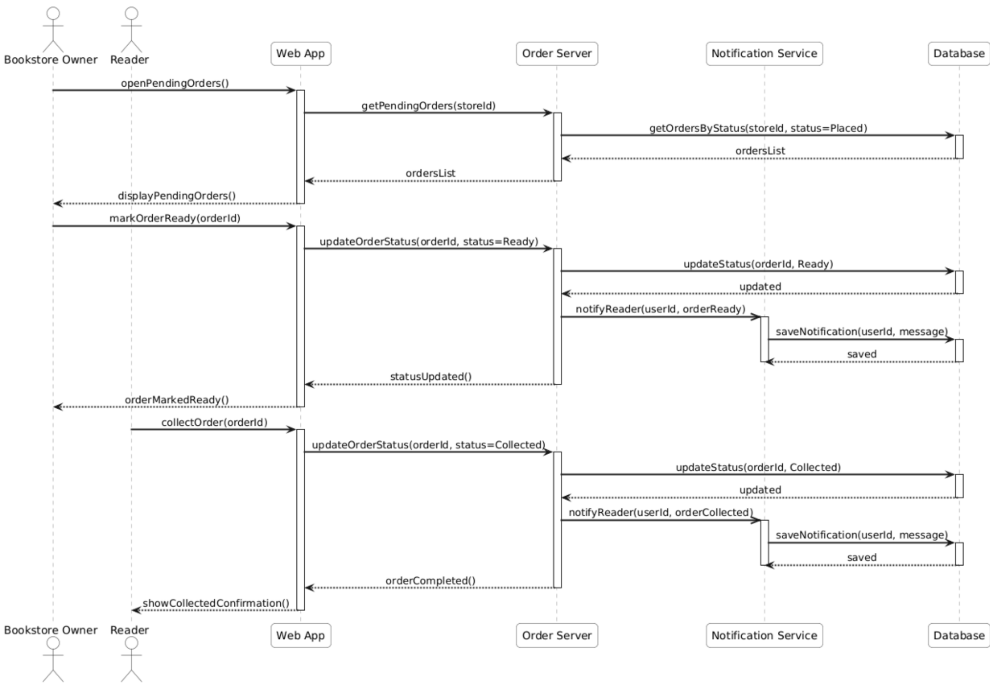
Sequence Diagram 03: Update Order Status
