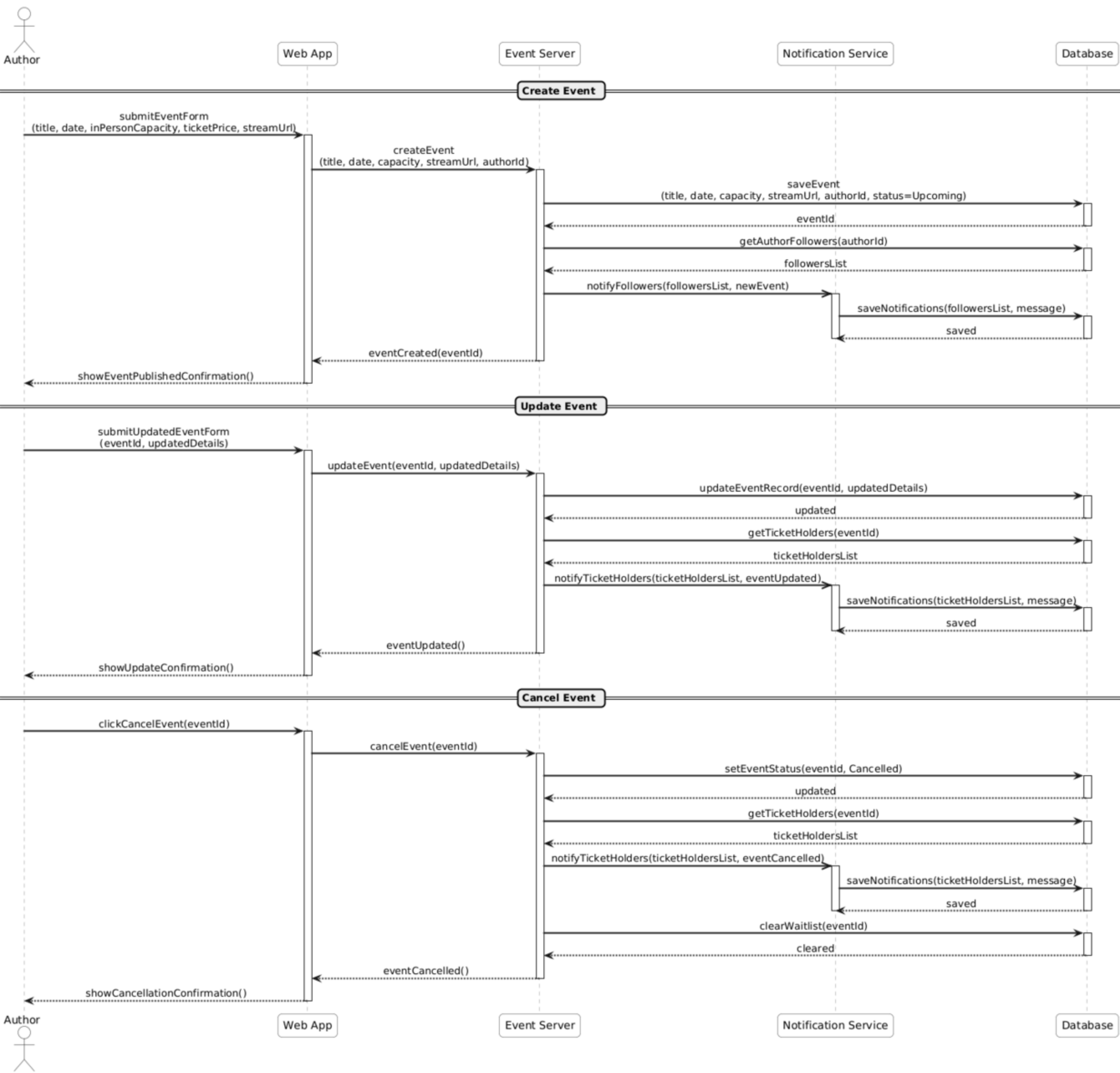
Sequence Diagram 13: Manage Events
