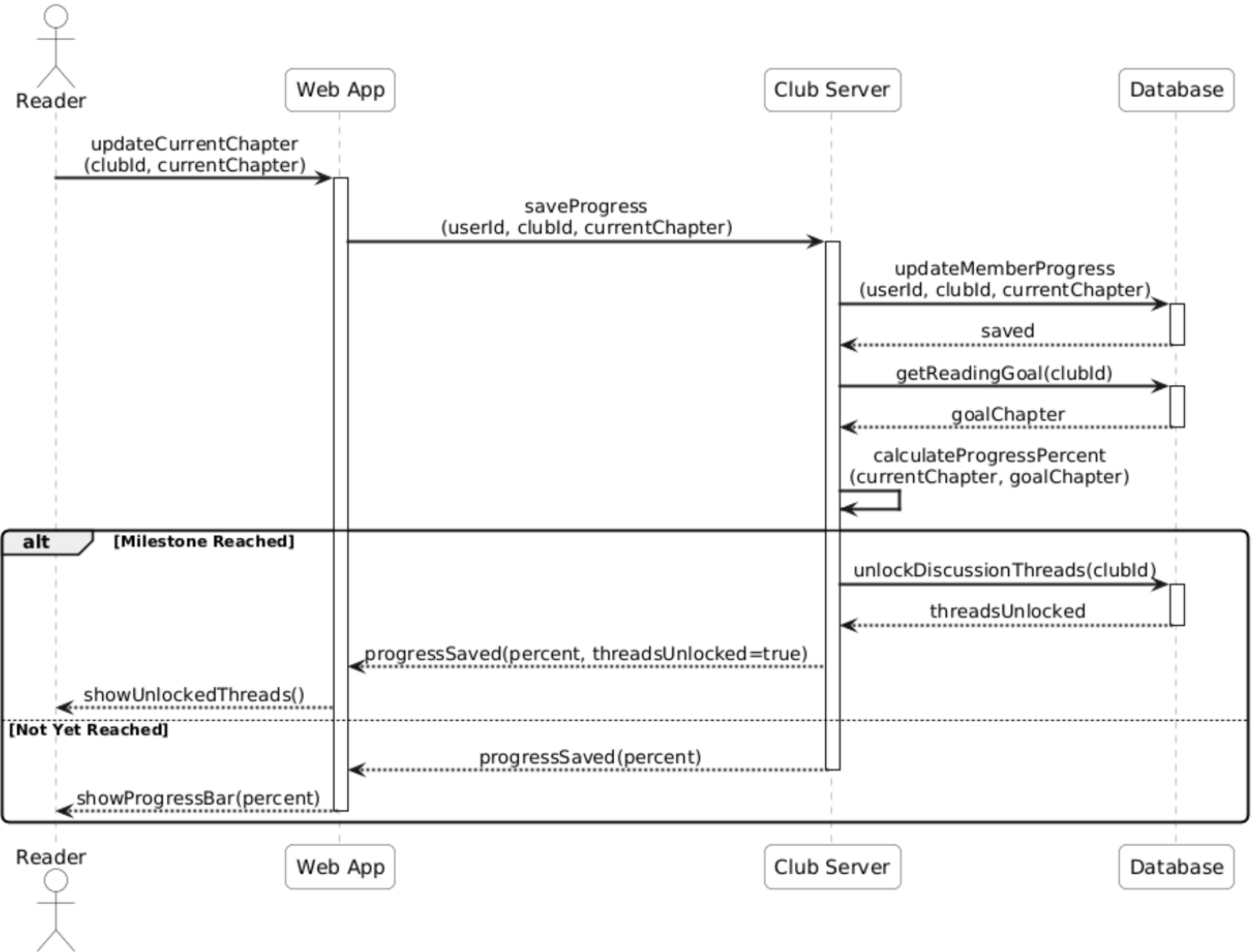
Sequence Diagram 09: Track Reading Progress
