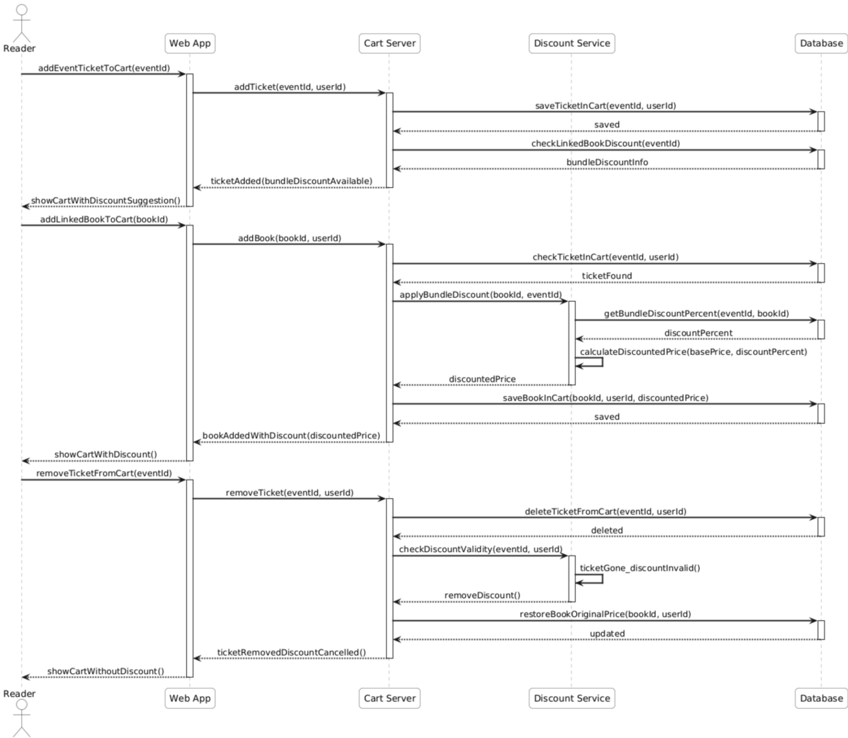
Sequence Diagram 19: Apply Bundle Discount
