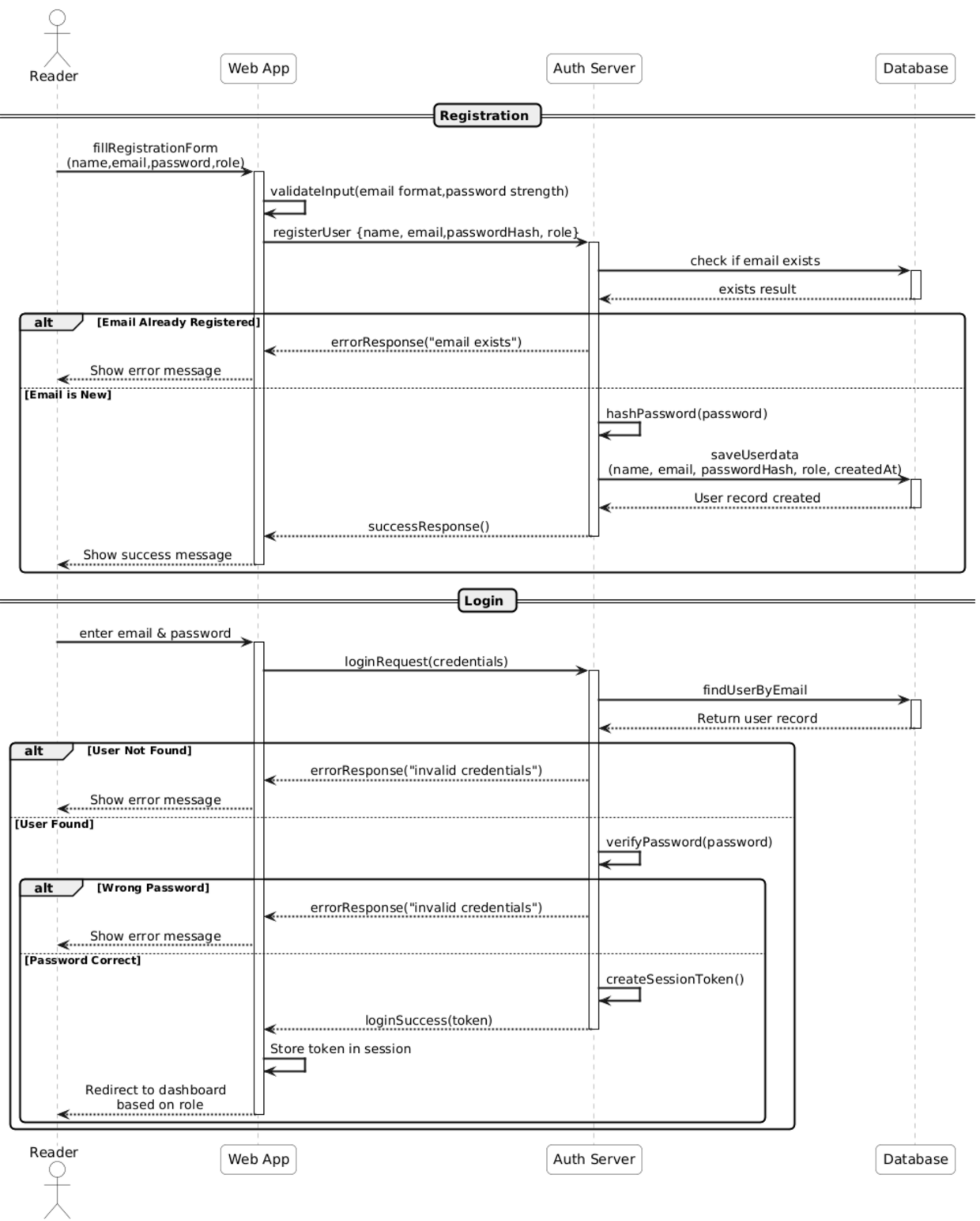
Sequence Diagram 01: User Registration and Login
