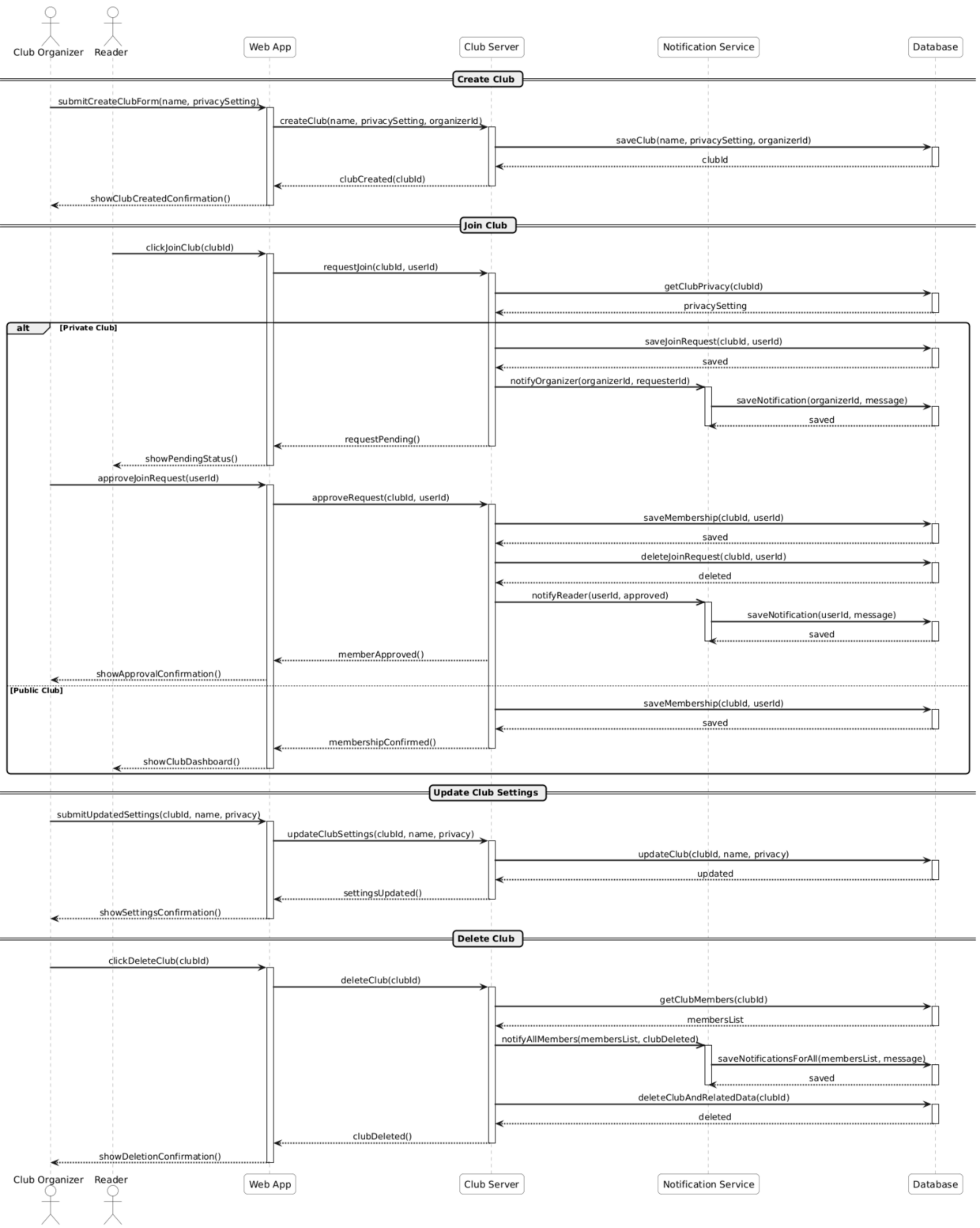
Sequence Diagram 07: Manage Book Club
