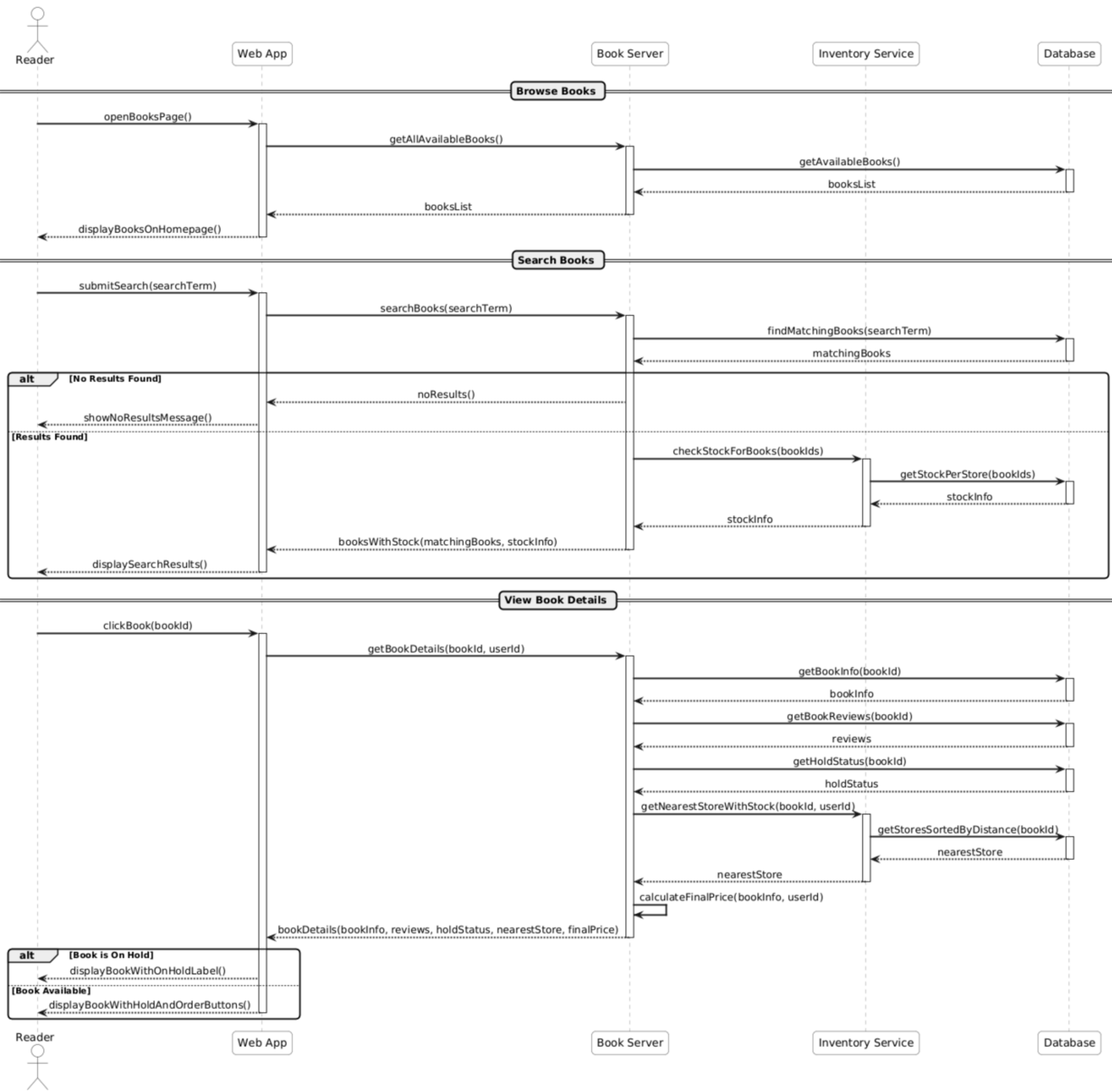
Sequence Diagram 18: Browse and Search Books
