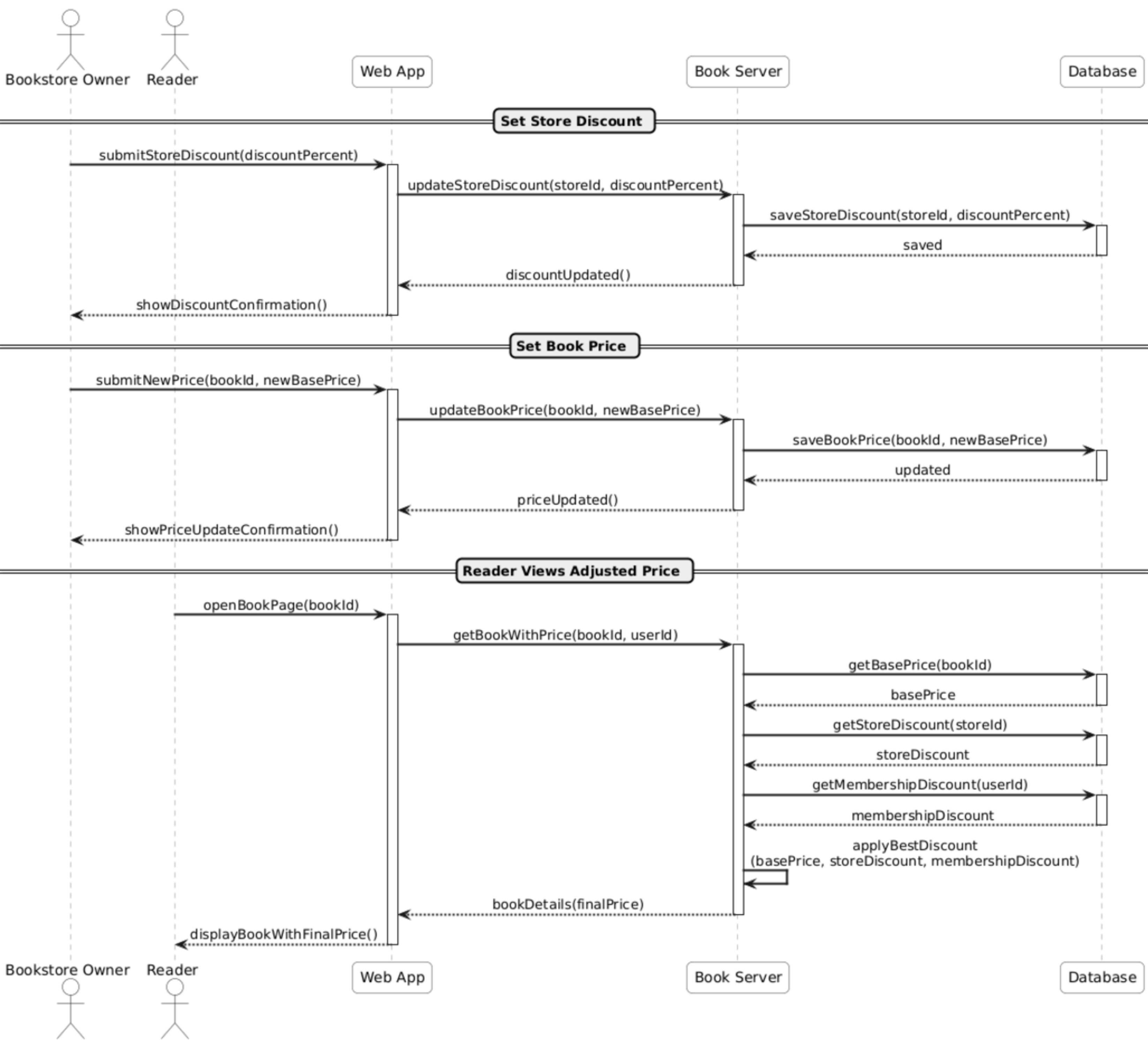
Sequence Diagram 06: Set Dynamic Price and Store Discount
