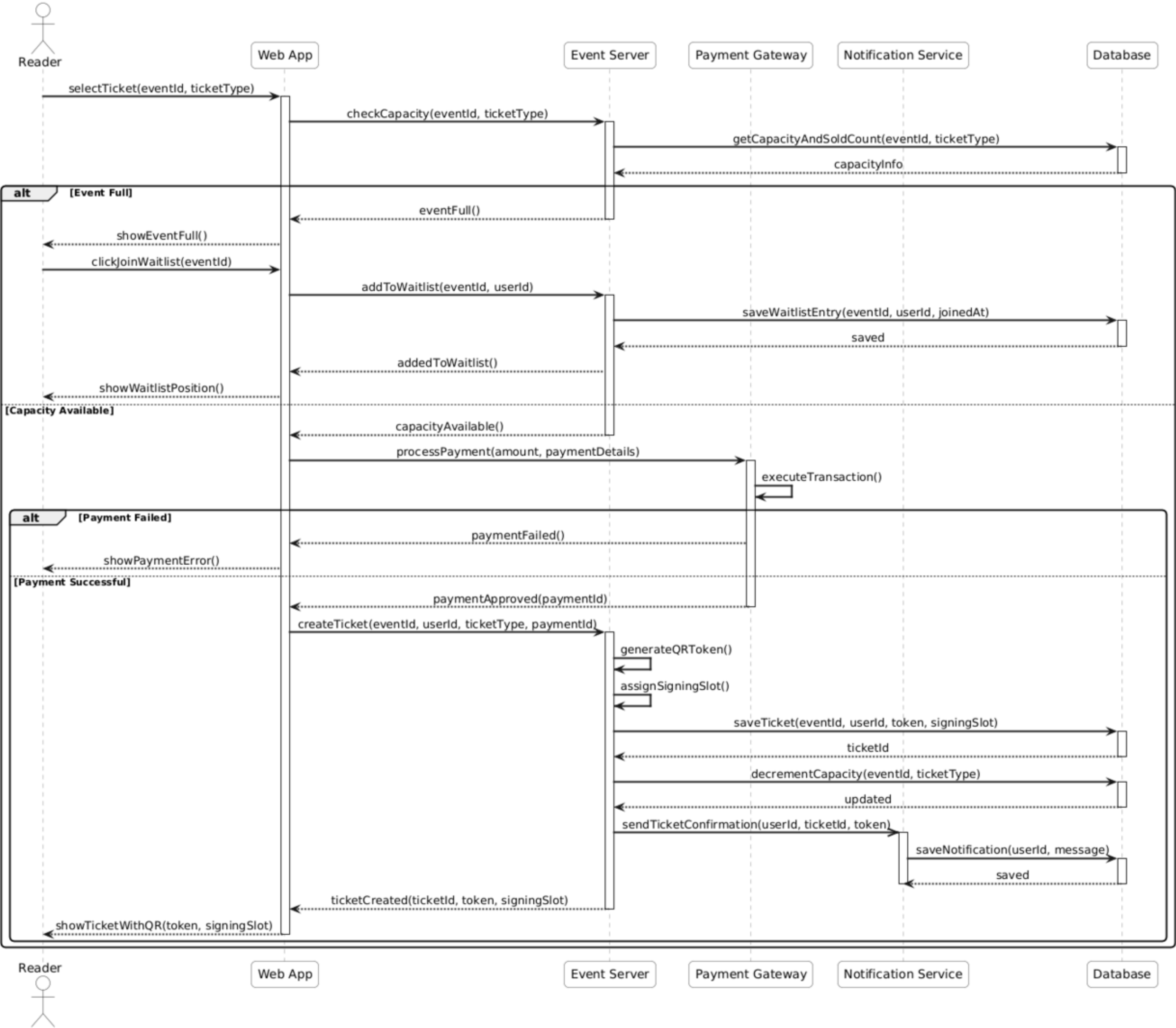
Sequence Diagram 14: Purchase Event Ticket and Join Waitlist
