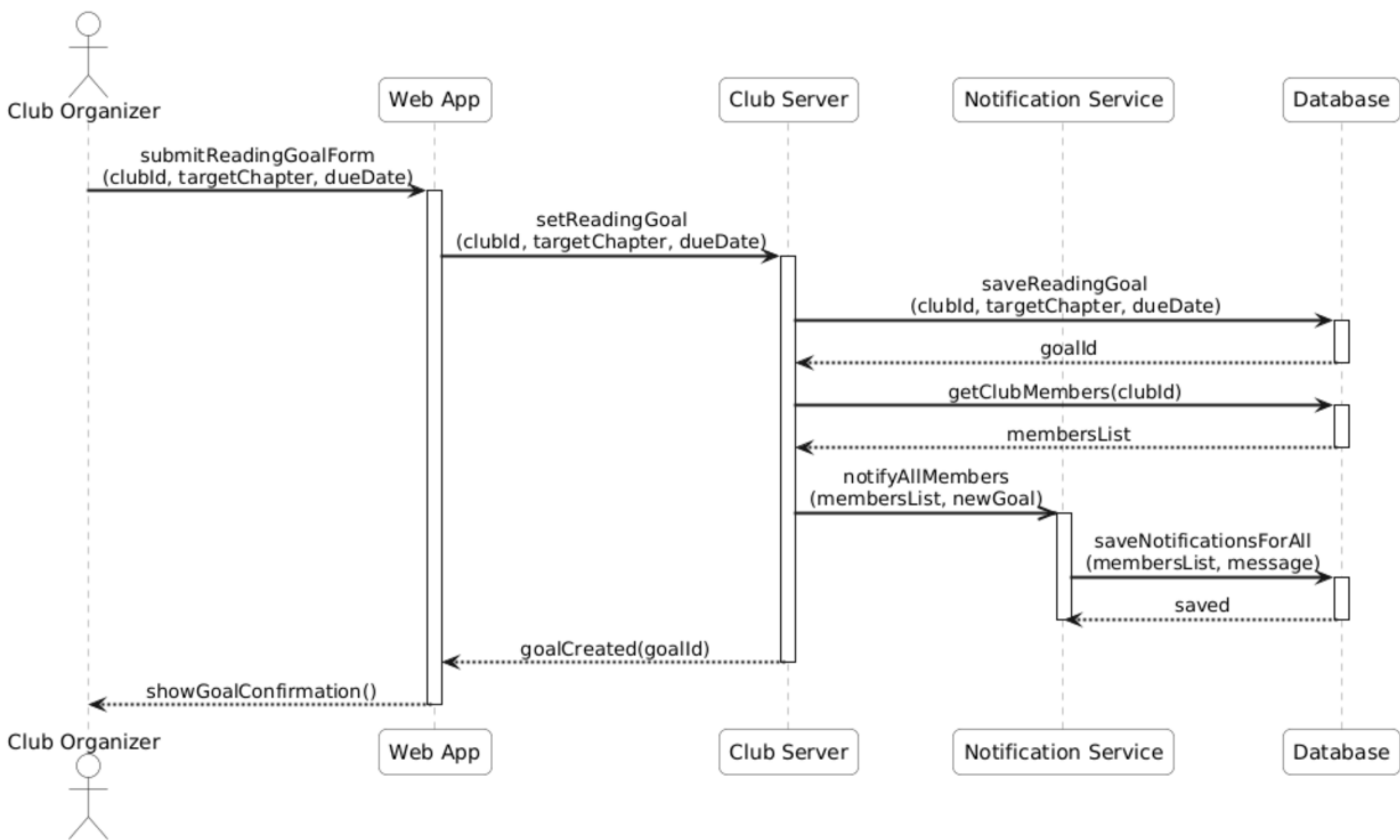
Sequence Diagram 08: Set Reading Schedule and Goals
