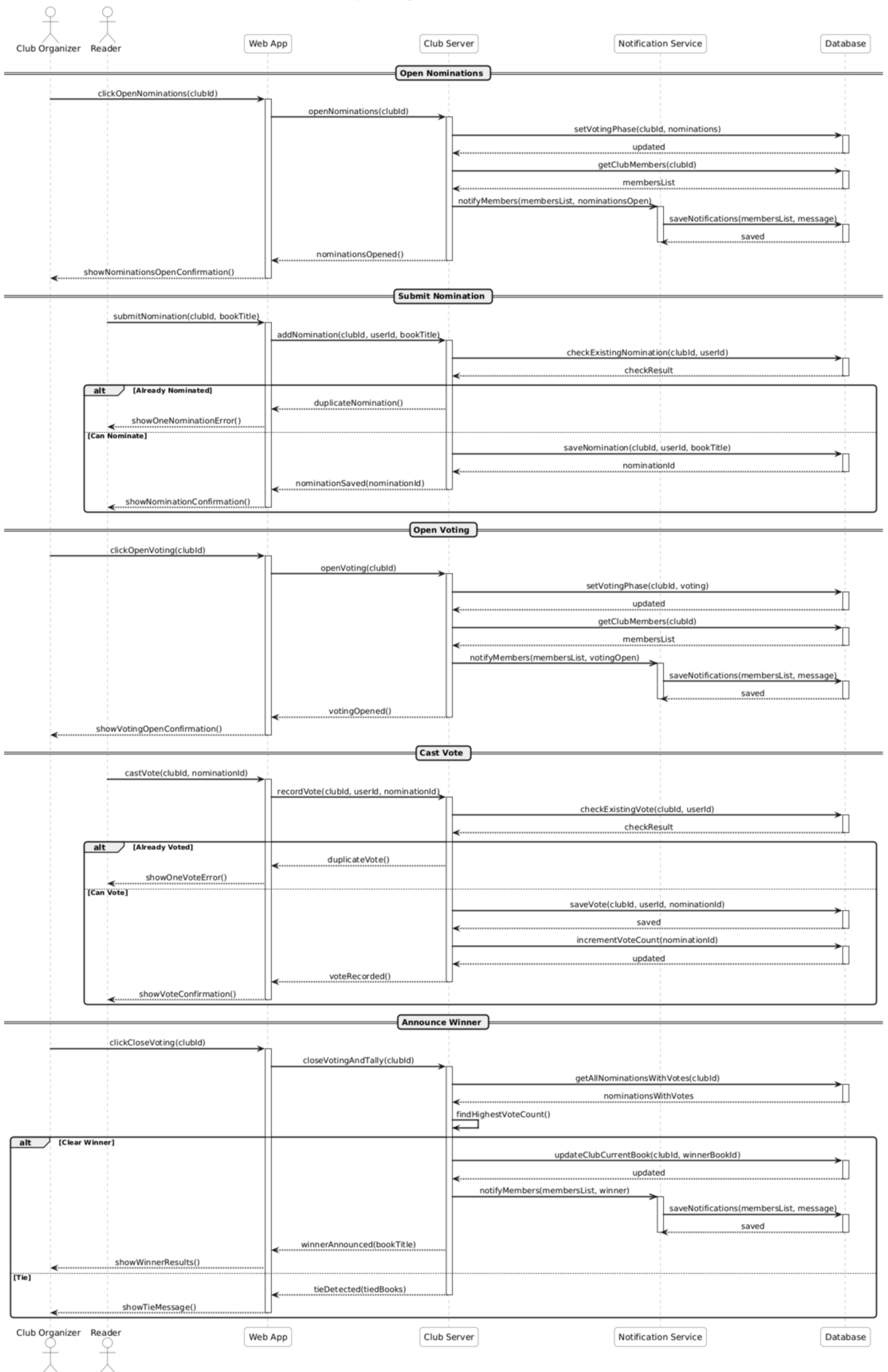
Sequence Diagram 11: Vote for Next Book
