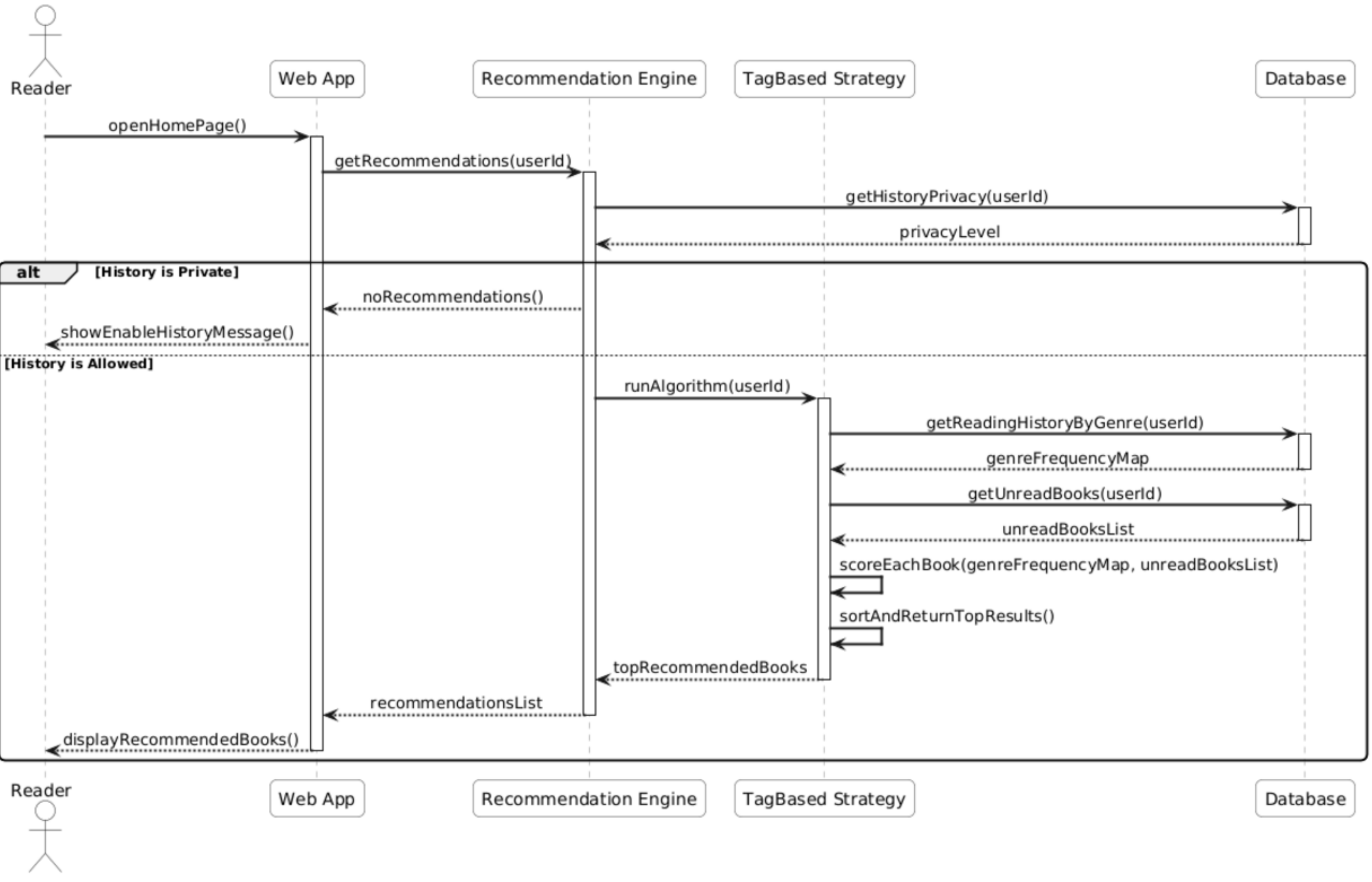
Sequence Diagram 17: View Book Recommendations
